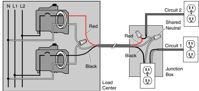
Figure 4: Example of Shared Neutral
