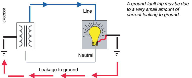
Figure 6: Diagram of a Ground Fault
