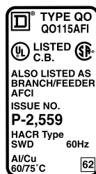
Branch/Feeder AFCI (Blue or Green Test Button)
