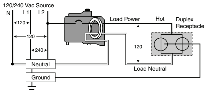
Figure 3: Example of Proper AFCI Wiring
